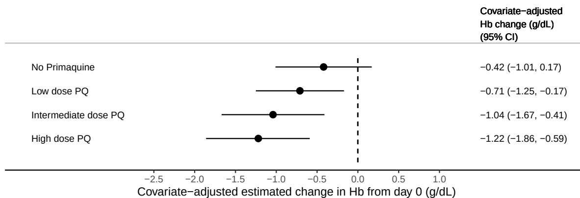
Figure 1_saf: The covariate-adjusted estimated change in Hb between primaquine daily dose groups on (A) days 2-3 and (B) days 5-7, in patients with \geq 30\% G6PD activity.
